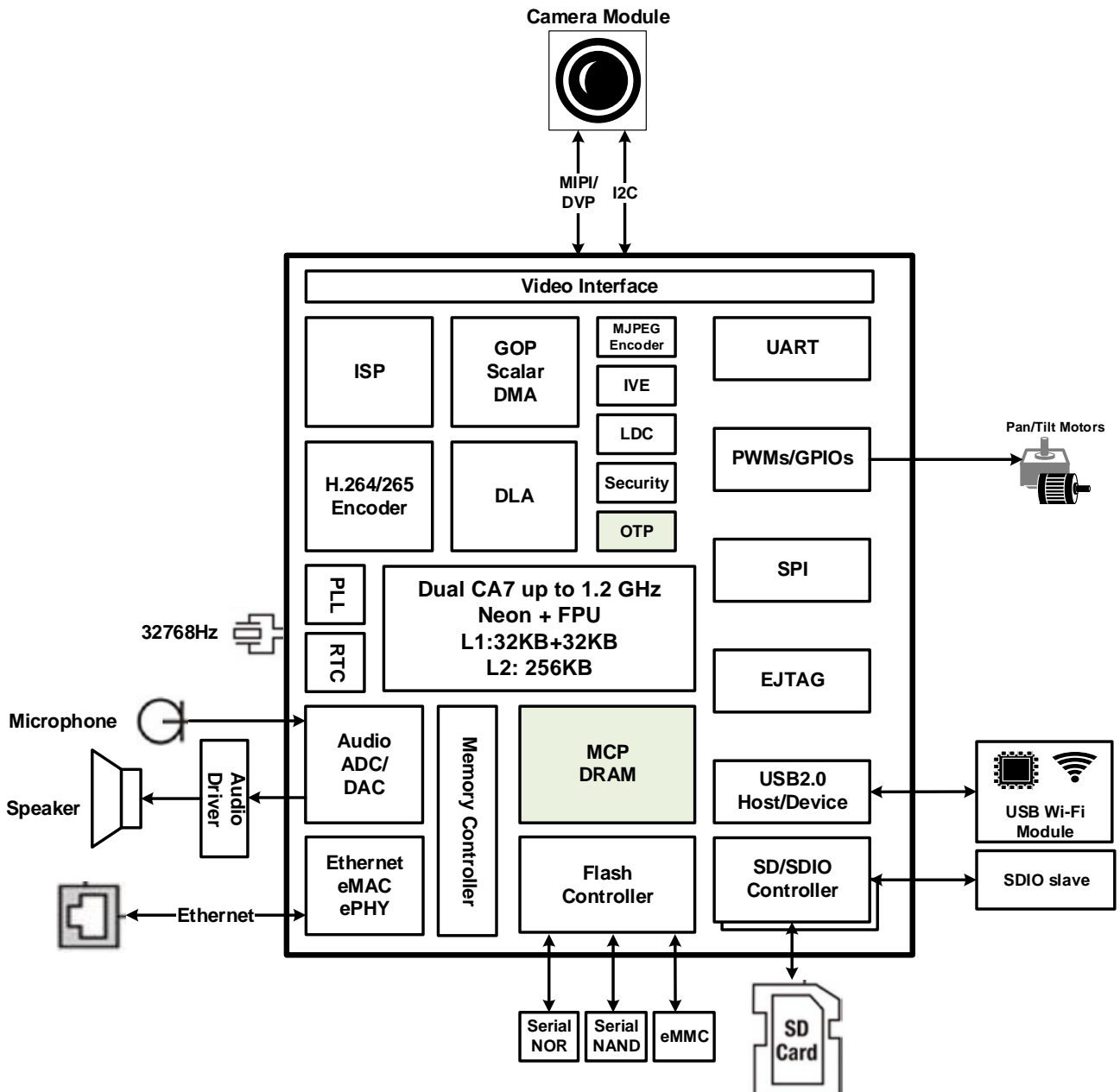
Figure 0-1: SSC338D/SSC338Q Block Diagram
